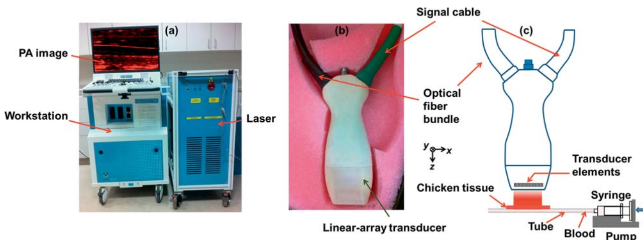
Figure 1 Photographs of the PAT system (a) and the linear-array-transducer (b). The workstation has a 64-channel data acquisition system, a data processing system, and an image display interface. (c) A schematic of the array in the phantom experiments.
